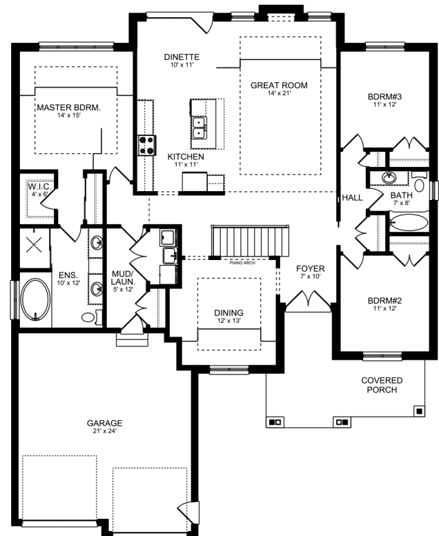
MAIN FLOOR PLAN AREA: 2017 SQ.FT.
