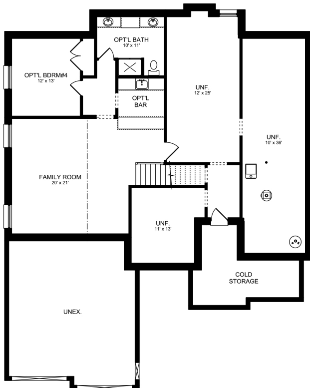
BASEMENT FLOOR PLAN FIN. AREA: 825 SQ.FT.
