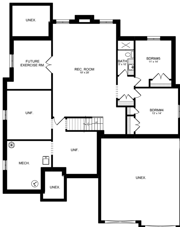
BASEMENT PLAN FIN. AREA: 1041 SQ.FT.
