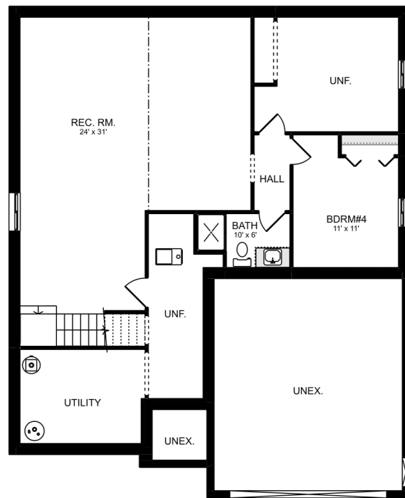
BASMENT PLAN
