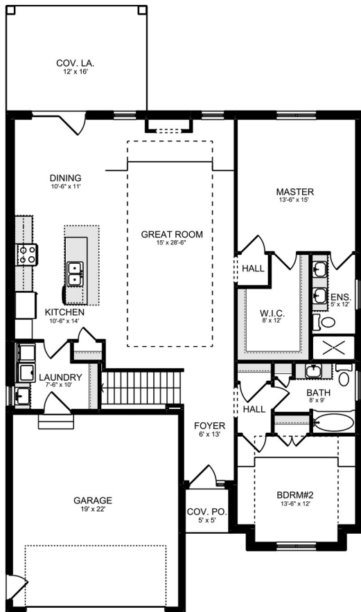
MAIN FLOOR PLAN AREA = 1,676 SQ.FT.
