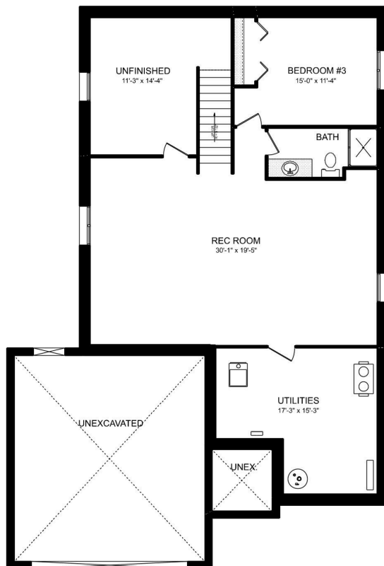
BASEMENT PLAN FINISHED AREA = 852 SQ.FT.
