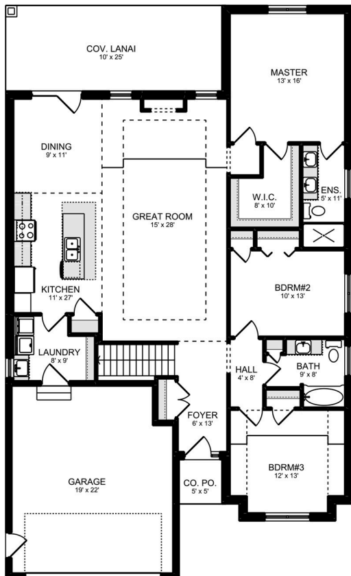
MAIN FLOOR PLAN AREA ~ 1,853 SQ.FT.
