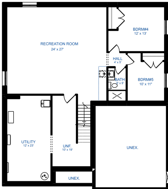
BASEMENT PLAN FINISHED AREA = 1044.8 Sq.ft
