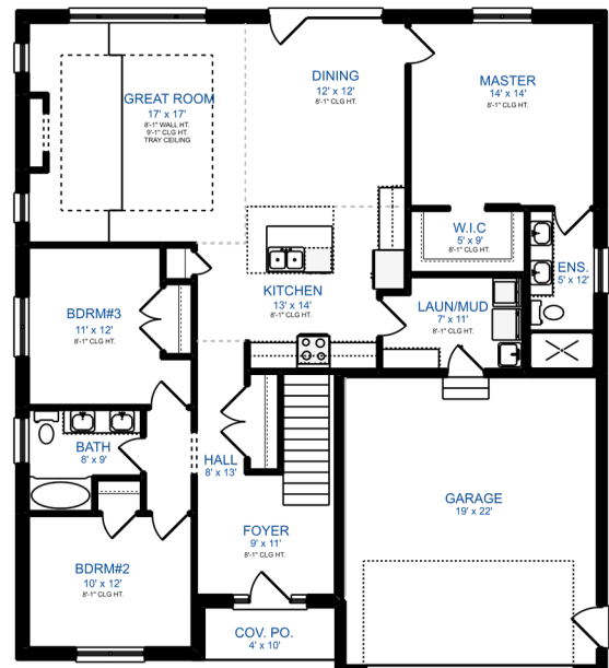
MAIN FLOOR PLAN AREA = 1752.5 Sq.ft
