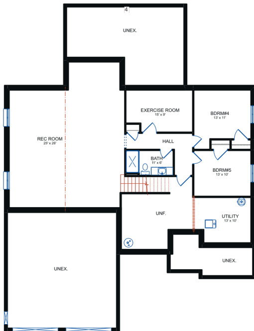
BASEMENT PLAN AREA: 1381.1 Sq. Ft. TOTAL WIDTH x LENGTH = 50'-0" x 73'-10"
