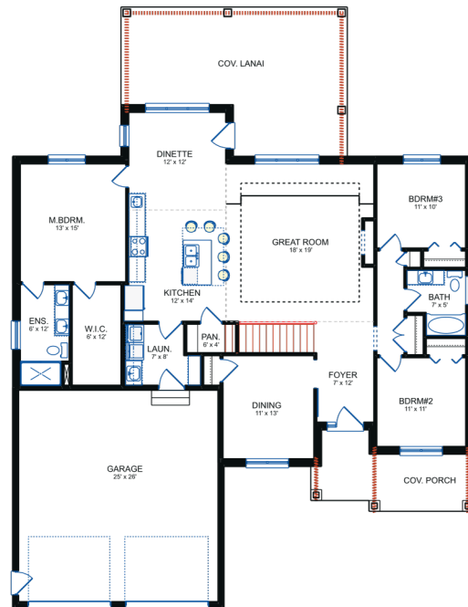
MAIN FLOOR PLAN AREA: 1865.2 Sq. Ft. TOTAL WIDTH x LENGTH = 50'-0" x 73'-10"
