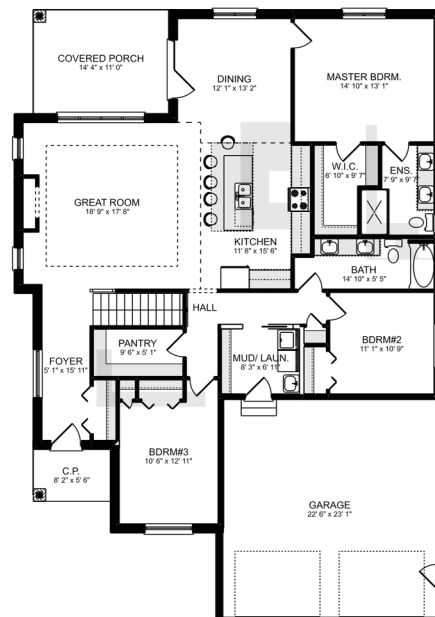
MAIN FLOOR PLAN AREA = 1880 sq. ft. TOTAL WIDTH x LENGTH = 45'-4" x 65'-0"
