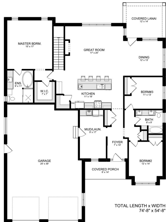
MAIN FLOOR PLAN AREA: 2163 Sq.ft.
