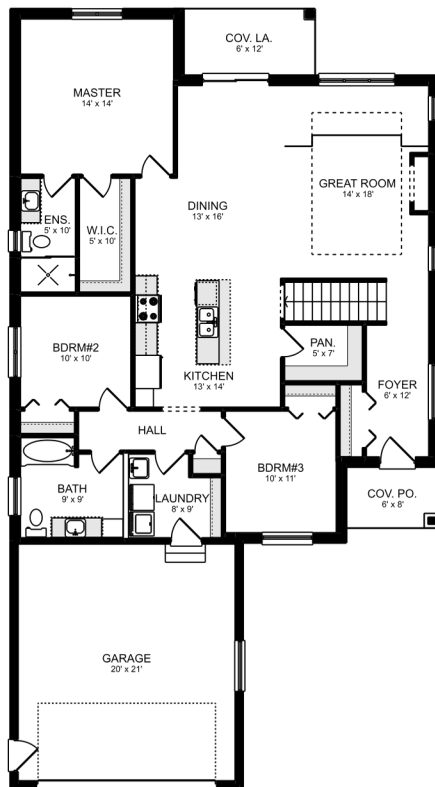
MAIN FLOOR PLAN AREA = 1668 Sq.ft.
