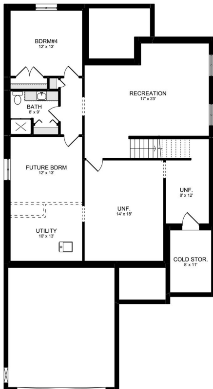
BASEMENT FLOOR PLAN FINISHED AREA = 682 Sq.ft.
